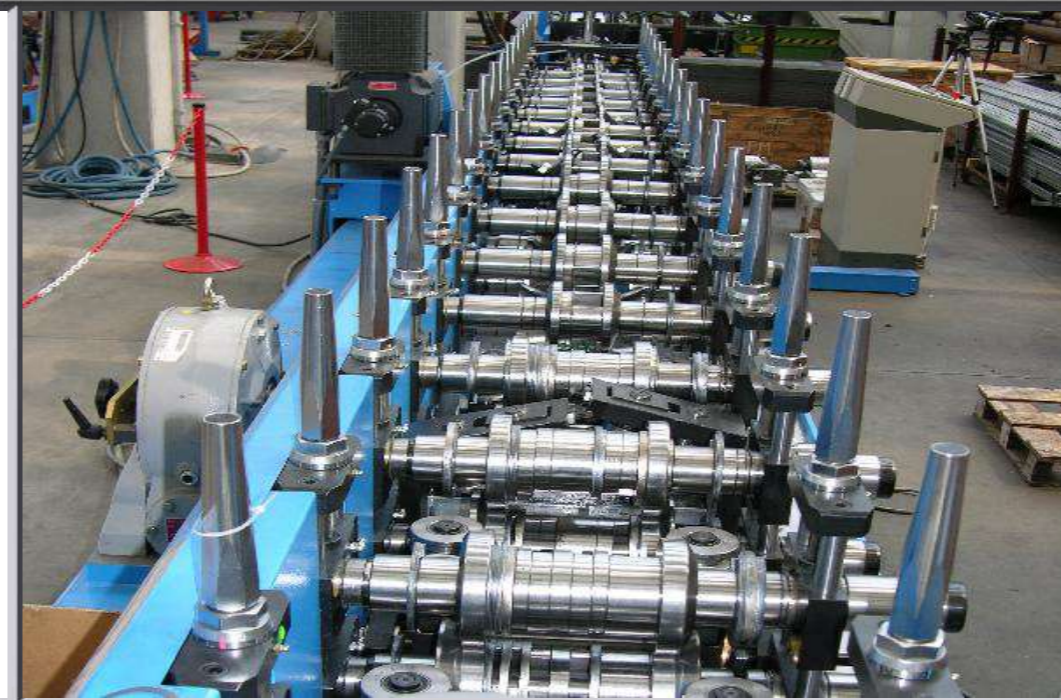
Photovoltaic profile roll forming
